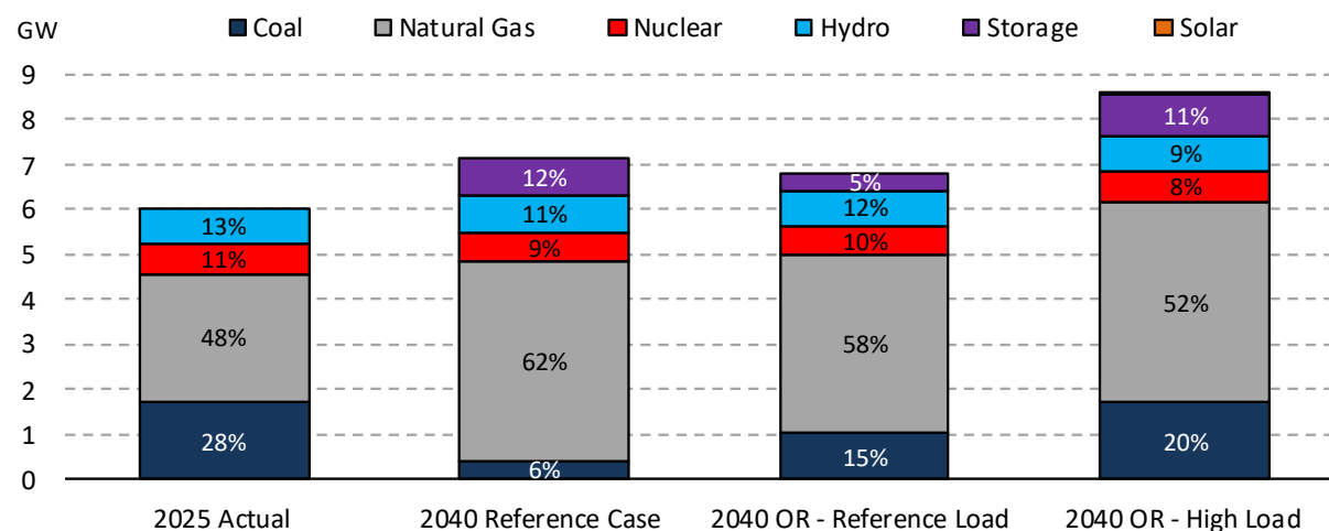
FIGURE ES-1: FIRM WINTER CAPACITY BY FUELTYPE
