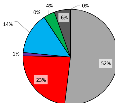
EXHIBIT 7: NORTHEAST - 2022 END-OF-YEAR CAPACITY MIX & FULL-YEAR GENERATION MIX BY FUEL TYPE
